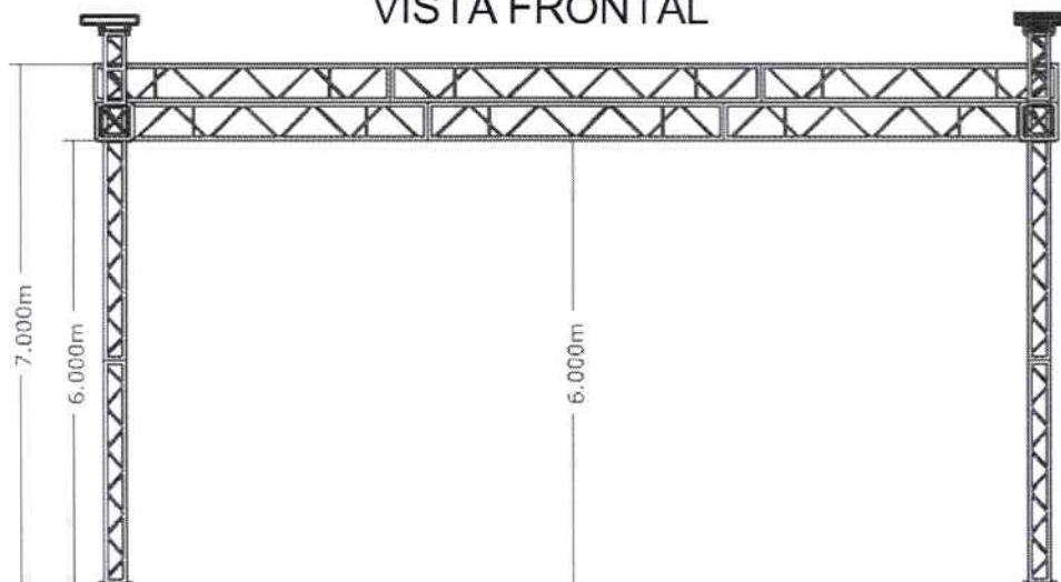
VISTA FRONTAL
